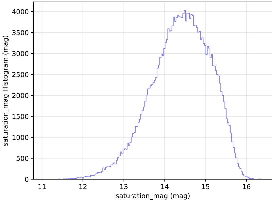
too_elab_heavy_r128_d3_griz_v3.4_10yrs All sky g band: saturation_mag Histogram
