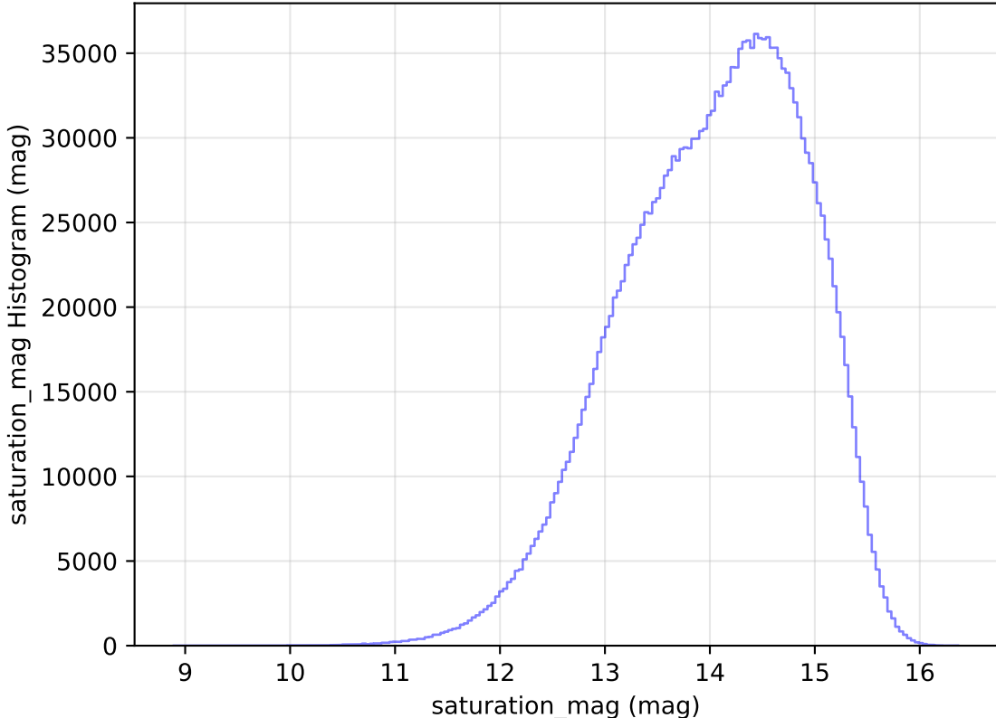
too_elab_heavy_r128_d3_griz_v3.4_10yrs All sky all bands: saturation_mag Histogram
