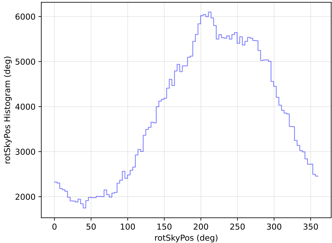
too_elab_heavy_r128_d3_griz_v3.4_10yrs WFD y band: rotSkyPos Histogram
