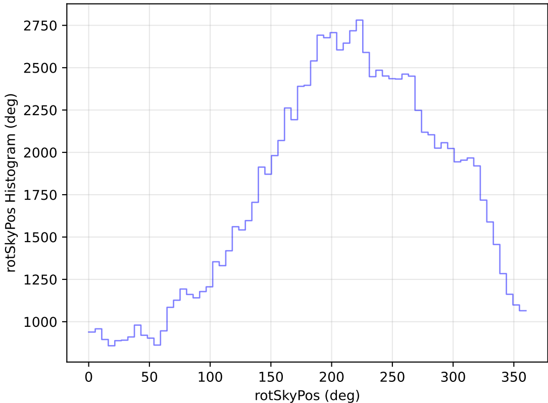
too_elab_heavy_r128_d3_griz_v3.4_10yrs WFD u band: rotSkyPos Histogram
