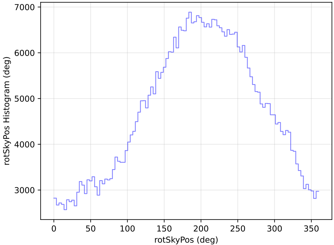
too_elab_heavy_r128_d3_griz_v3.4_10yrs WFD r band: rotSkyPos Histogram
