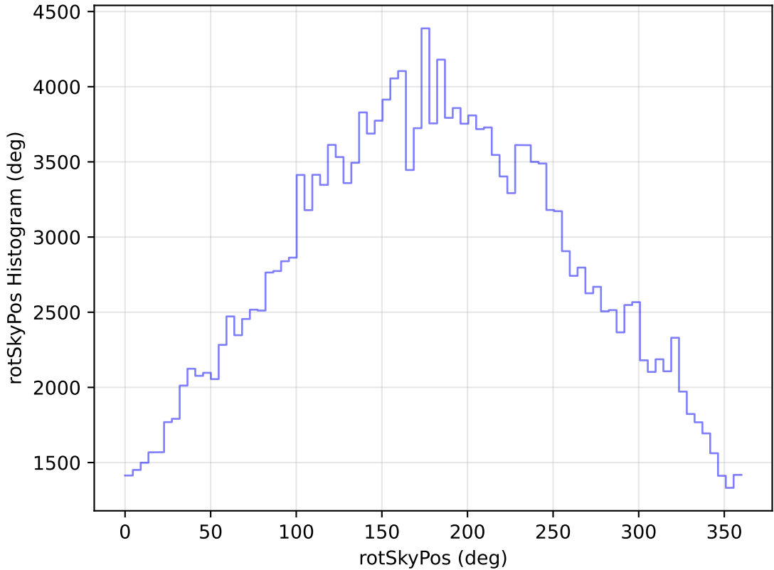
too_elab_heavy_r128_d3_griz_v3.4_10yrs WFD g band: rotSkyPos Histogram
