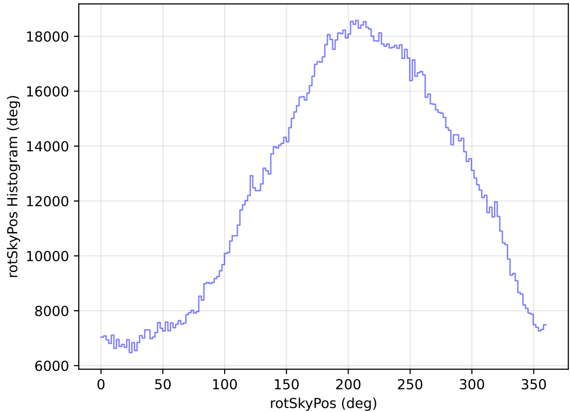
too_elab_heavy_r128_d3_griz_v3.4_10yrs WFD all bands: rotSkyPos Histogram
