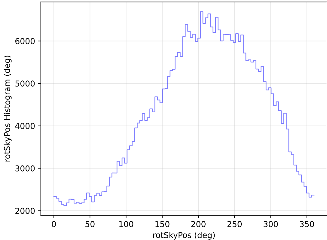
too_elab_heavy_r128_d3_griz_v3.4_10yrs All sky z band: rotSkyPos Histogram
