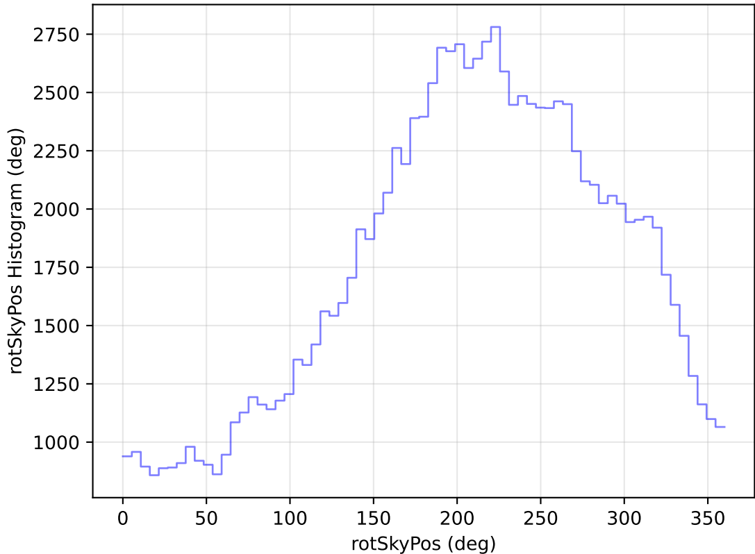
too_elab_heavy_r128_d3_griz_v3.4_10yrs All sky u band: rotSkyPos Histogram
