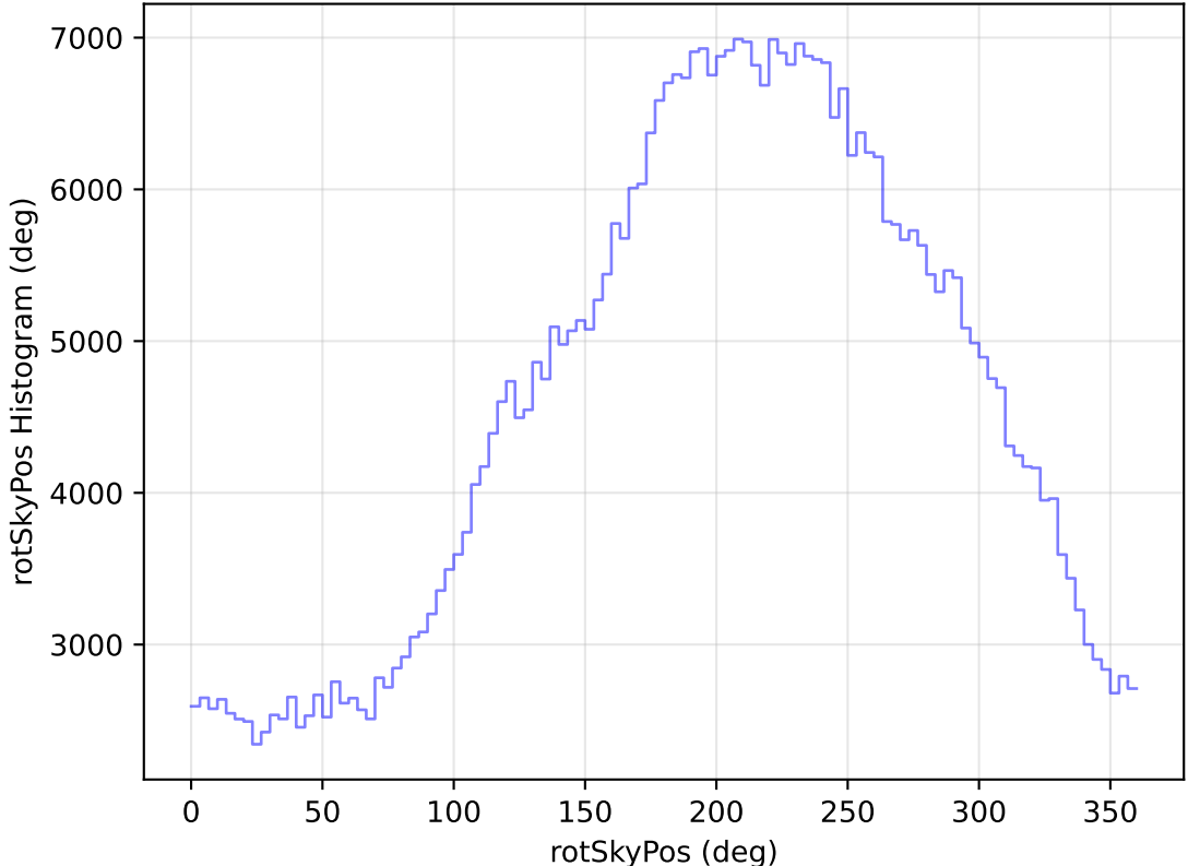
too_elab_heavy_r128_d3_griz_v3.4_10yrs All sky i band: rotSkyPos Histogram
