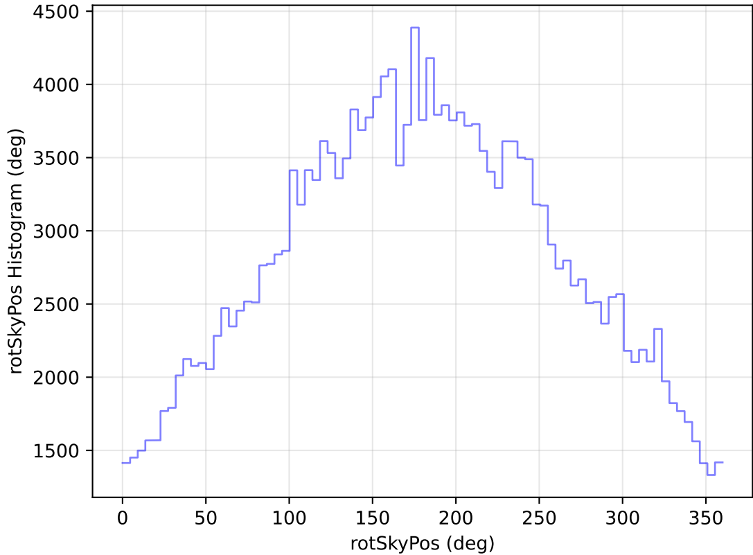
too_elab_heavy_r128_d3_griz_v3.4_10yrs All sky g band: rotSkyPos Histogram
