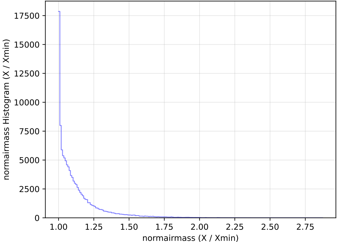
too_elab_heavy_r128_d3_griz_v3.4_10yrs WFD u band: normairmass Histogram
