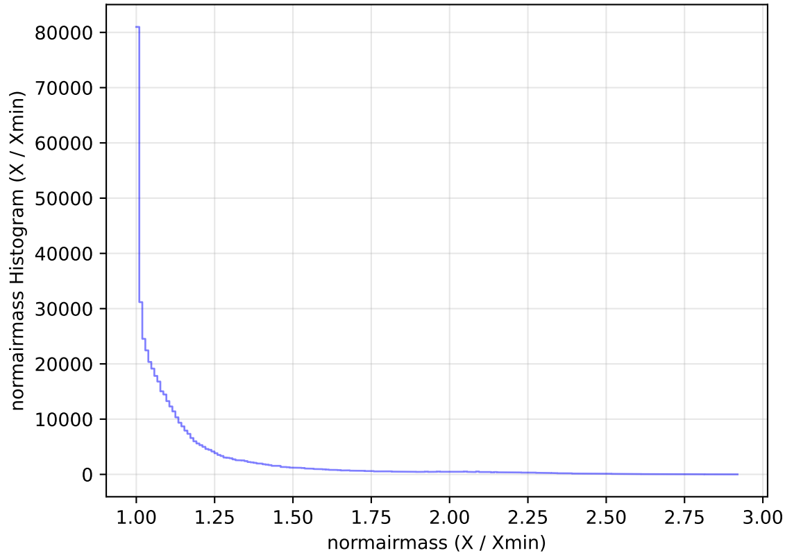
too_elab_heavy_r128_d3_griz_v3.4_10yrs WFD i band: normairmass Histogram
