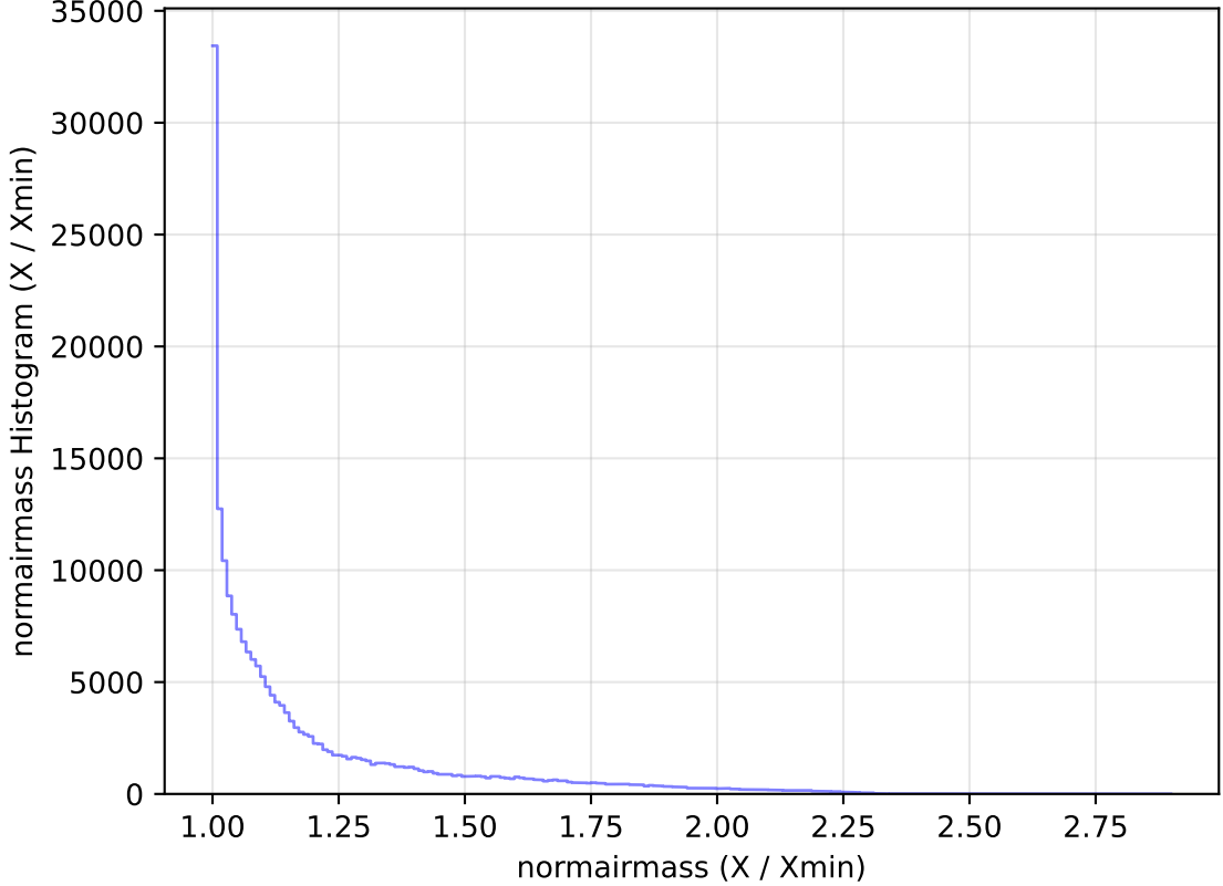
too_elab_heavy_r128_d3_griz_v3.4_10yrs WFD g band: normairmass Histogram
