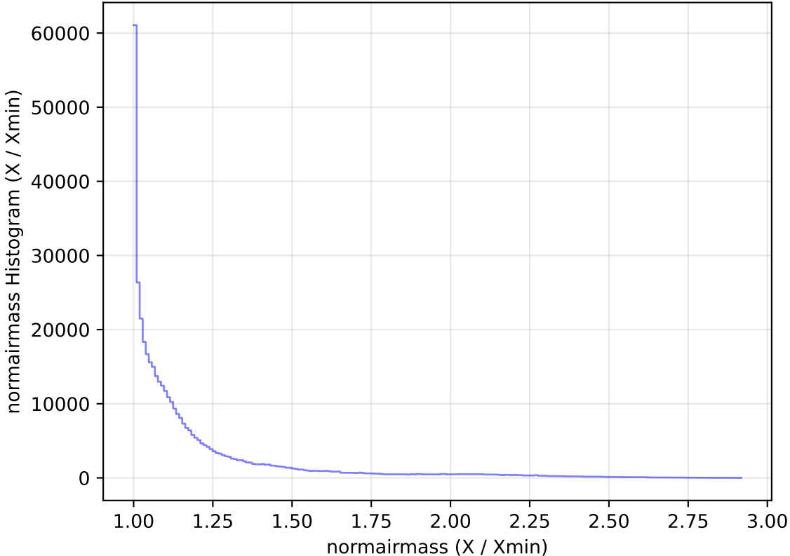
too_elab_heavy_r128_d3_griz_v3.4_10yrs All sky z band: normairmass Histogram
