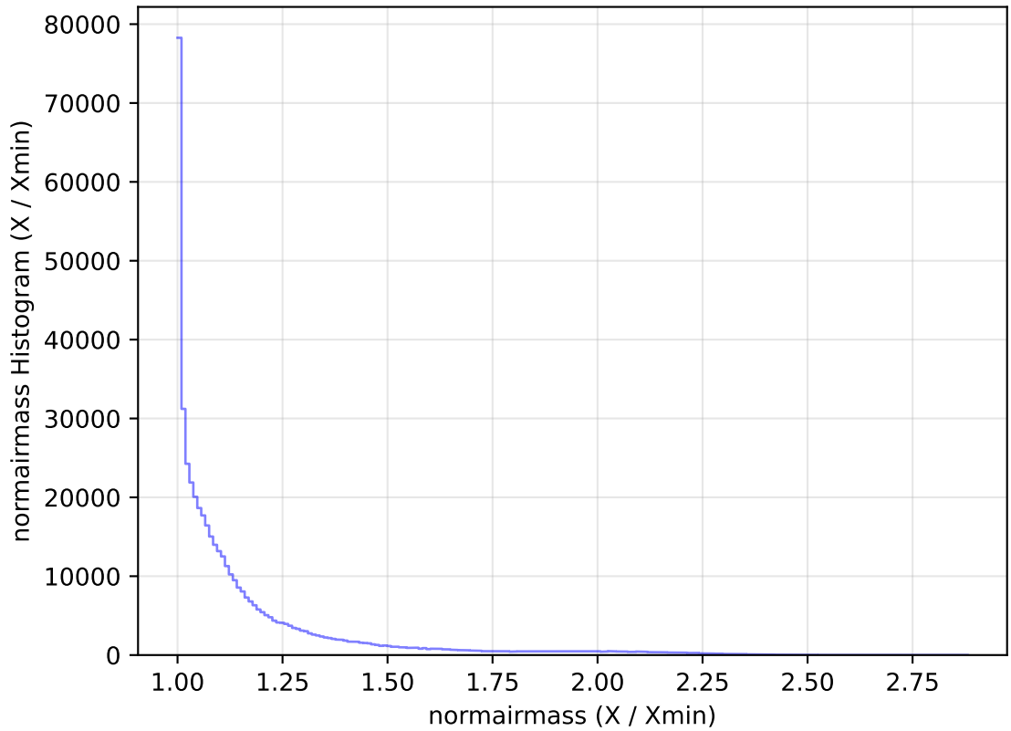
too_elab_heavy_r128_d3_griz_v3.4_10yrs All sky r band: normairmass Histogram
