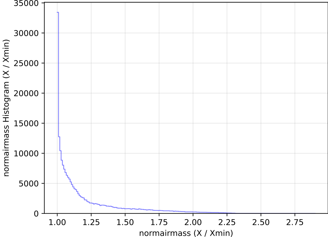
too_elab_heavy_r128_d3_griz_v3.4_10yrs All sky g band: normairmass Histogram
