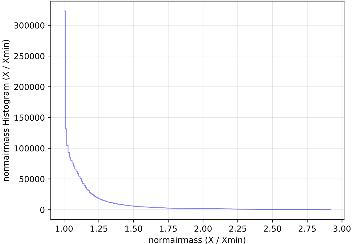
too_elab_heavy_r128_d3_griz_v3.4_10yrs All sky all bands: normairmass Histogram
