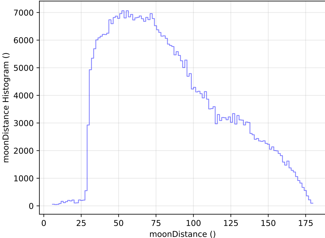
too_elab_heavy_r128_d3_griz_v3.4_10yrs WFD z band: moonDistance Histogram
