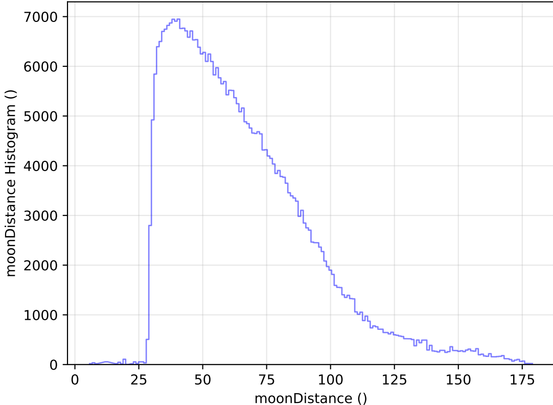
too_elab_heavy_r128_d3_griz_v3.4_10yrs WFD y band: moonDistance Histogram
