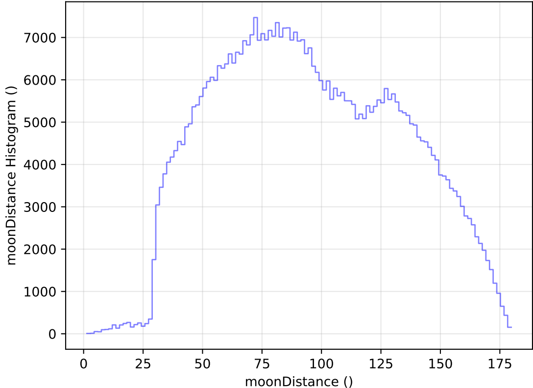
too_elab_heavy_r128_d3_griz_v3.4_10yrs WFD i band: moonDistance Histogram
