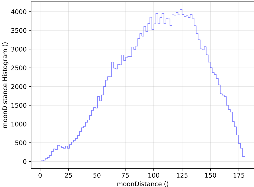
too_elab_heavy_r128_d3_griz_v3.4_10yrs WFD g band: moonDistance Histogram
