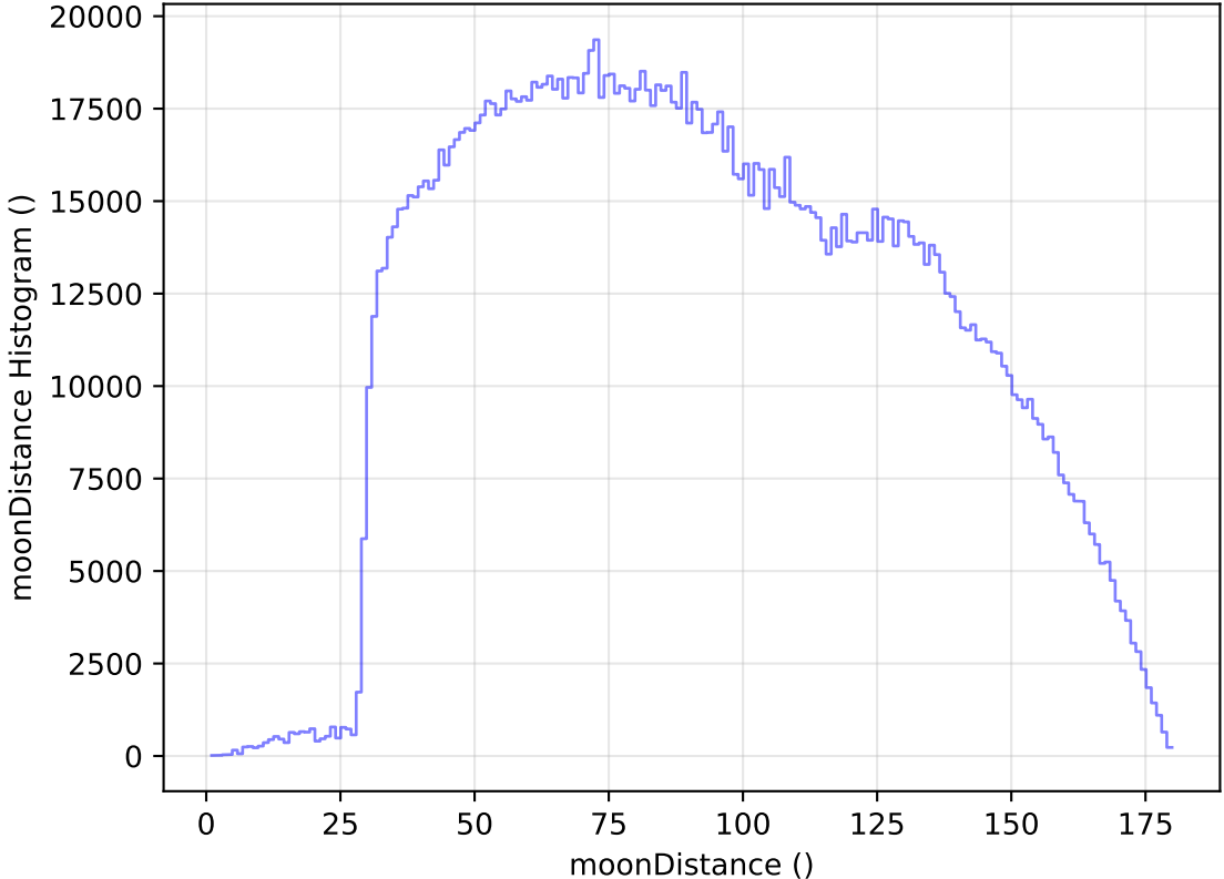
too_elab_heavy_r128_d3_griz_v3.4_10yrs WFD all bands: moonDistance Histogram
