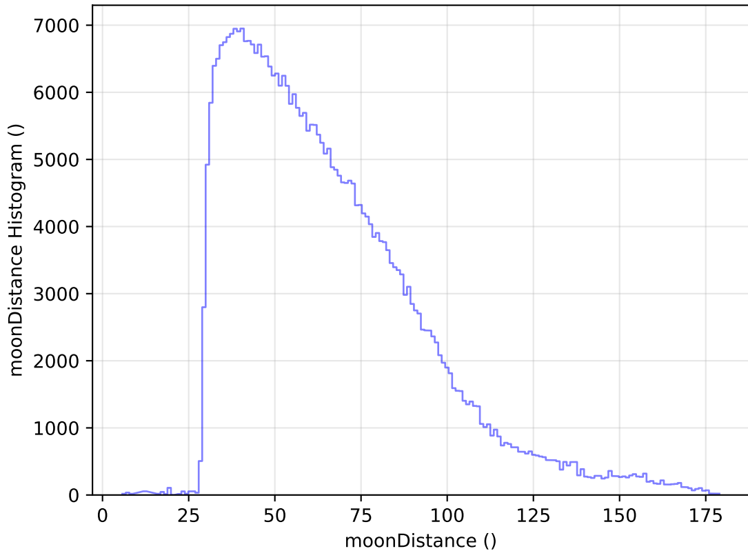
too_elab_heavy_r128_d3_griz_v3.4_10yrs All sky y band: moonDistance Histogram
