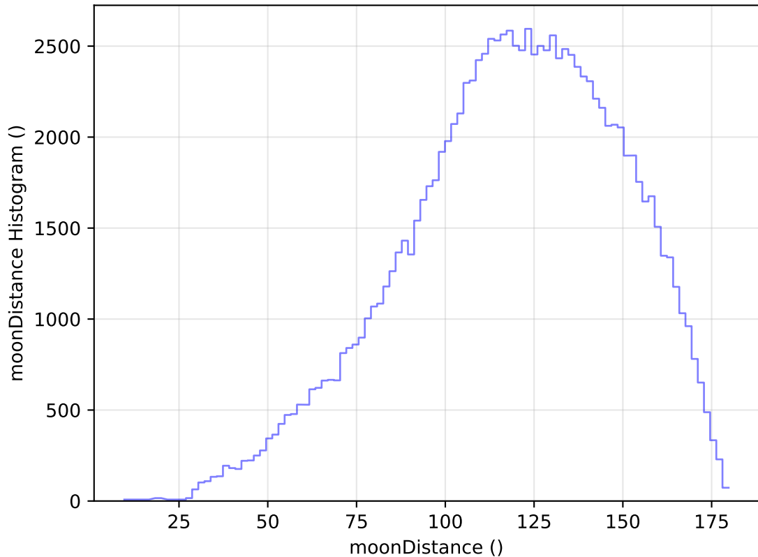
too_elab_heavy_r128_d3_griz_v3.4_10yrs All sky u band: moonDistance Histogram
