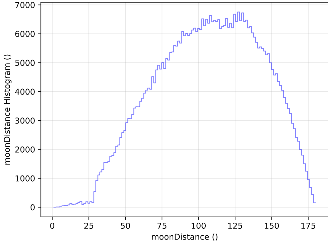
too_elab_heavy_r128_d3_griz_v3.4_10yrs All sky r band: moonDistance Histogram
