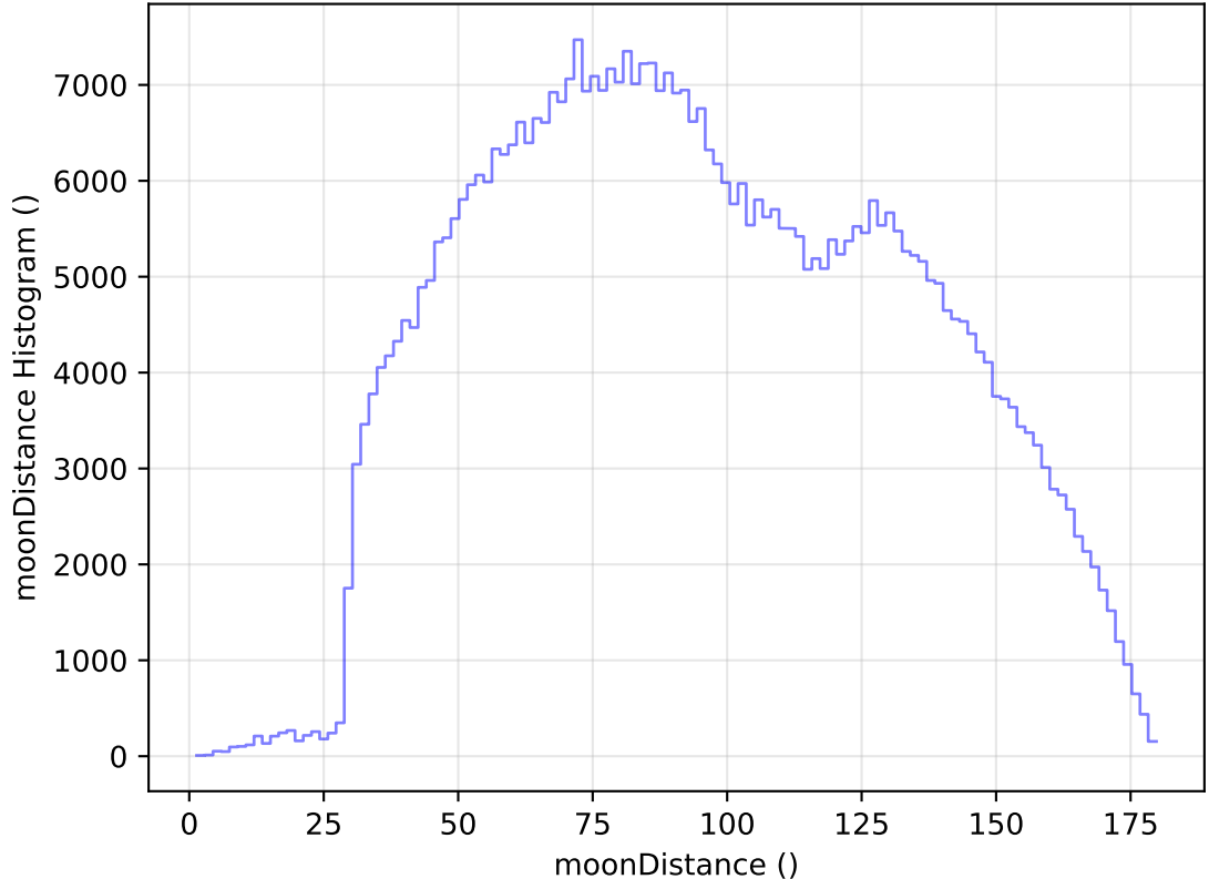
too_elab_heavy_r128_d3_griz_v3.4_10yrs All sky i band: moonDistance Histogram
