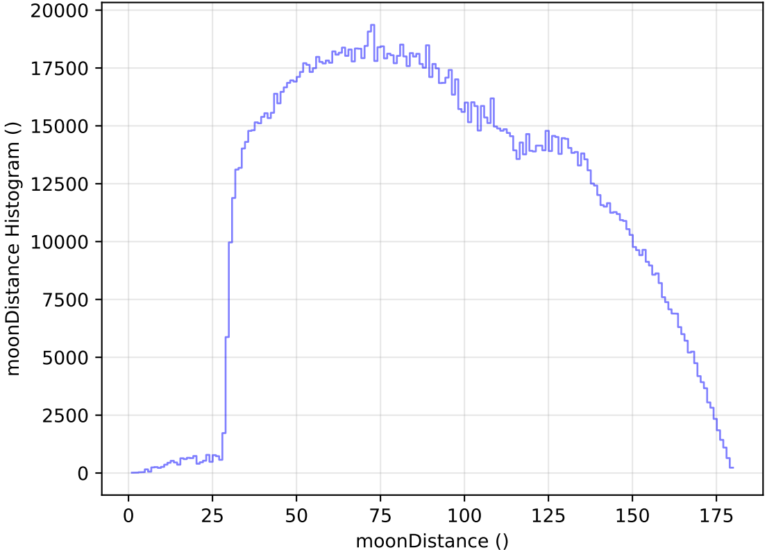
too_elab_heavy_r128_d3_griz_v3.4_10yrs All sky all bands: moonDistance Histogram
