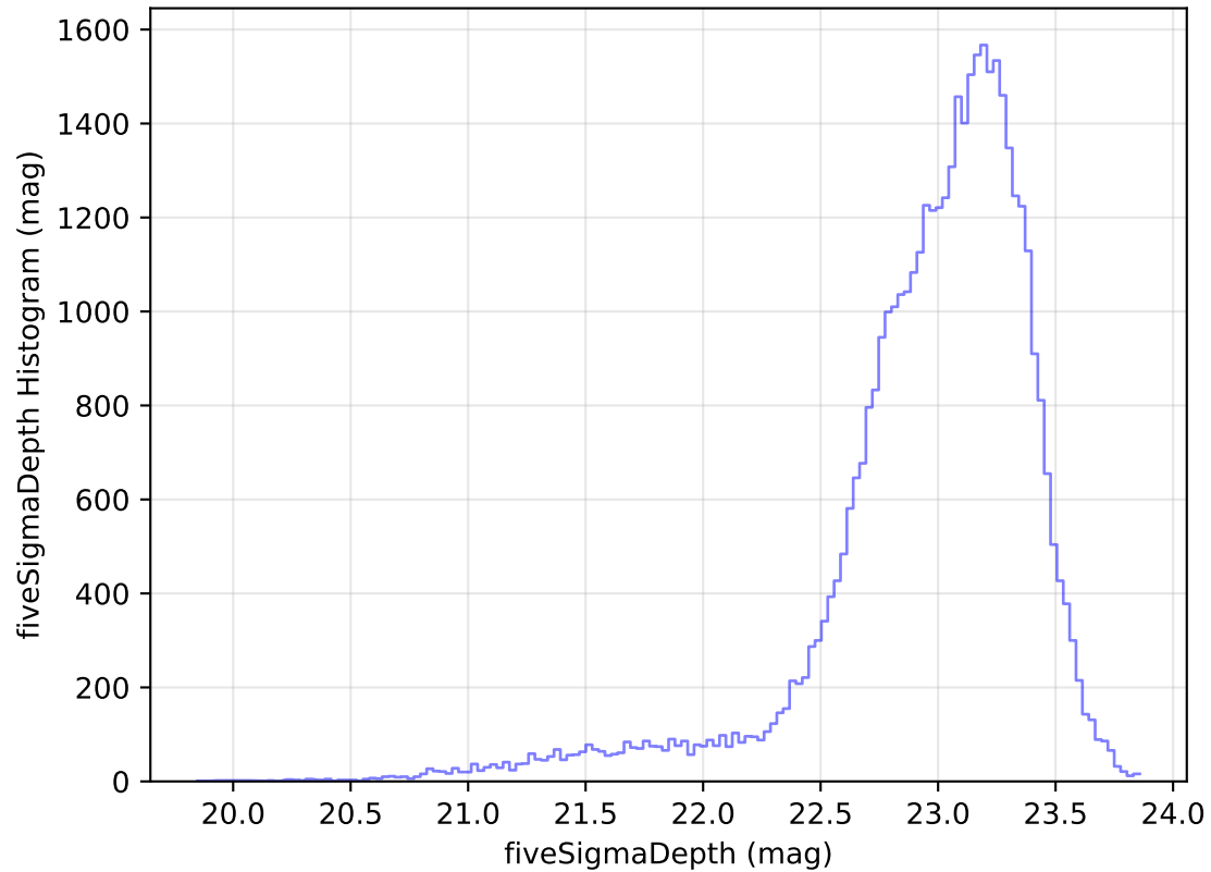
too_elab_heavy_r128_d3_griz_v3.4_10yrs Yr 1 z band: fiveSigmaDepth Histogram
