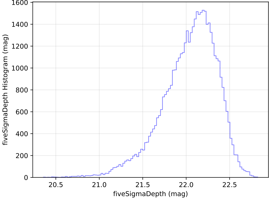
too_elab_heavy_r128_d3_griz_v3.4_10yrs Yr 1 y band: fiveSigmaDepth Histogram
