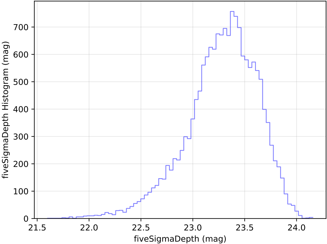
too_elab_heavy_r128_d3_griz_v3.4_10yrs Yr 1 u band: fiveSigmaDepth Histogram
