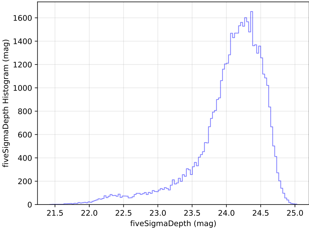
too_elab_heavy_r128_d3_griz_v3.4_10yrs Yr 1 r band: fiveSigmaDepth Histogram
