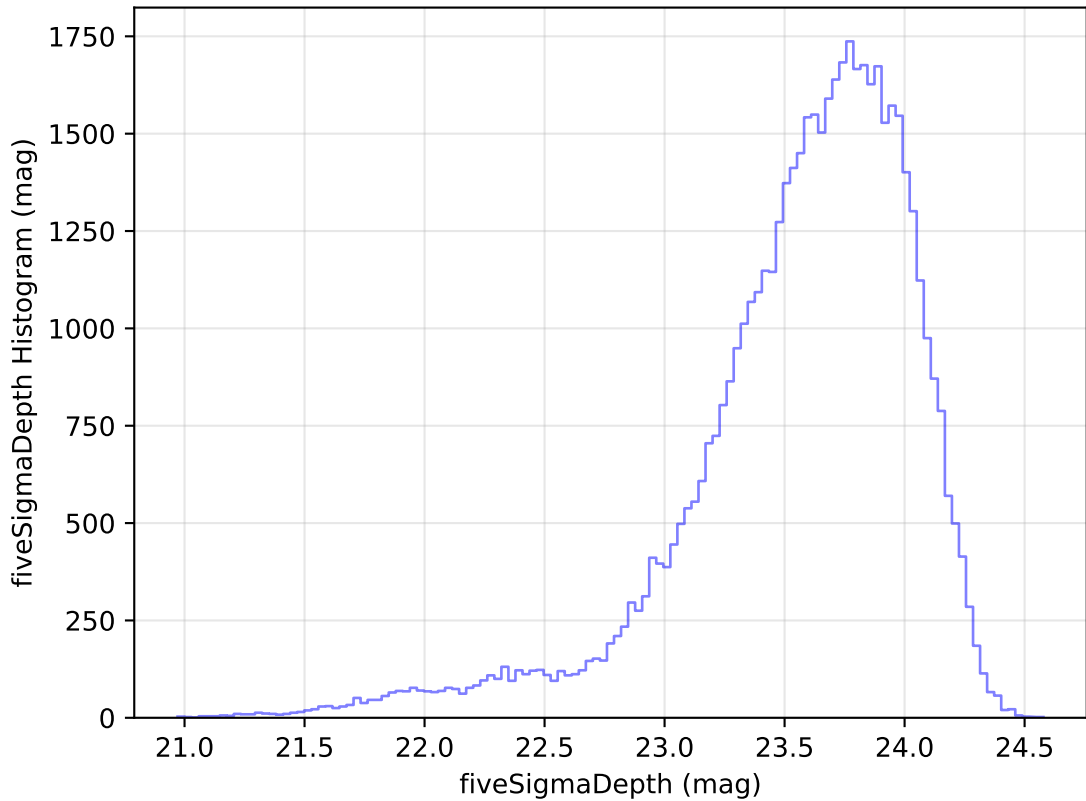
too_elab_heavy_r128_d3_griz_v3.4_10yrs Yr 1 i band: fiveSigmaDepth Histogram
