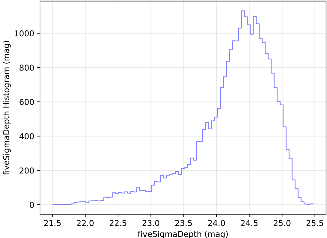
too_elab_heavy_r128_d3_griz_v3.4_10yrs Yr 1 g band: fiveSigmaDepth Histogram
