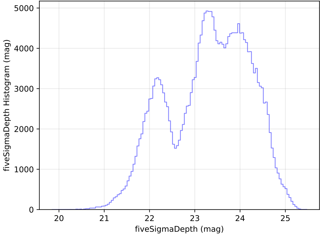
too_elab_heavy_r128_d3_griz_v3.4_10yrs Yr 1 all bands: fiveSigmaDepth Histogram
