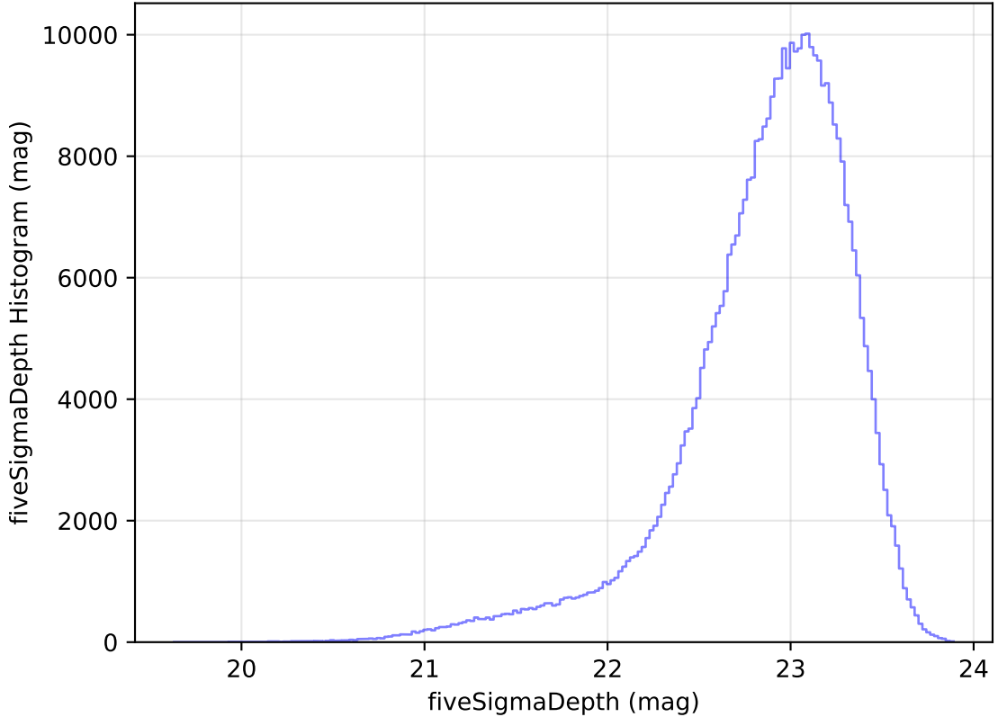
too_elab_heavy_r128_d3_griz_v3.4_10yrs WFD z band: fiveSigmaDepth Histogram
