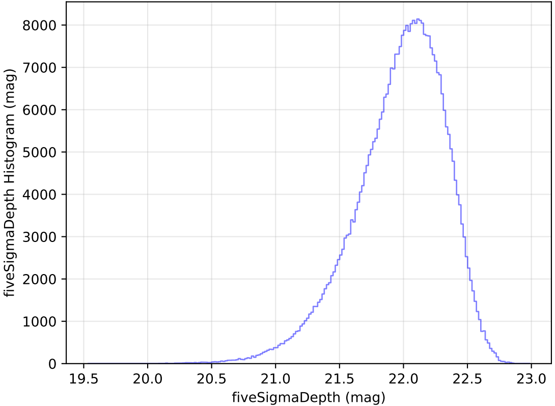
too_elab_heavy_r128_d3_griz_v3.4_10yrs WFD y band: fiveSigmaDepth Histogram
