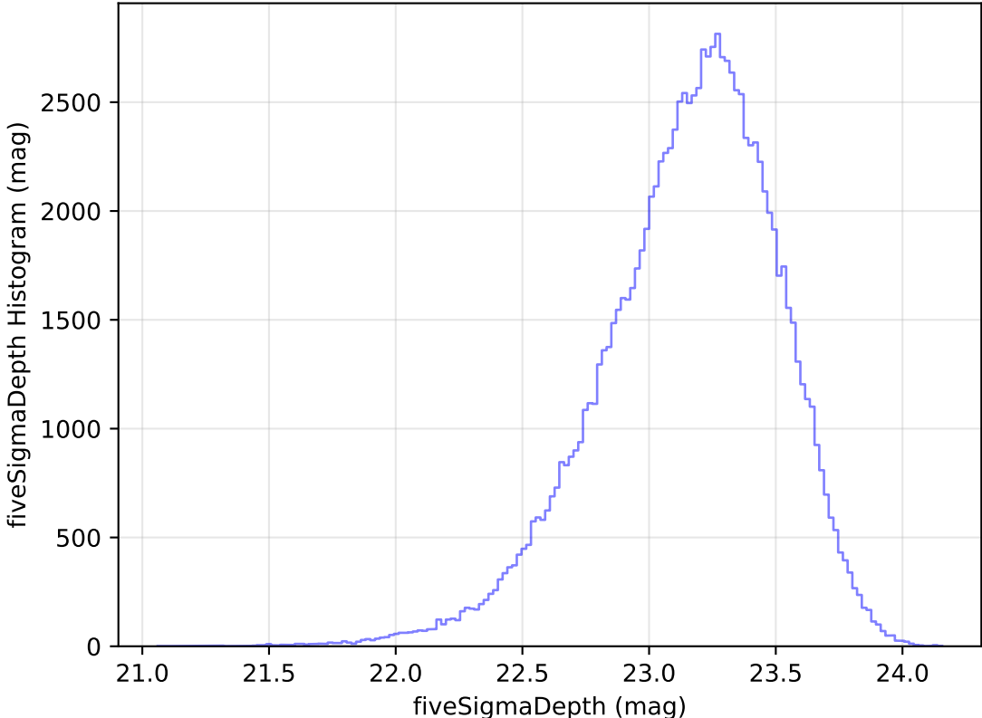
too_elab_heavy_r128_d3_griz_v3.4_10yrs WFD u band: fiveSigmaDepth Histogram
