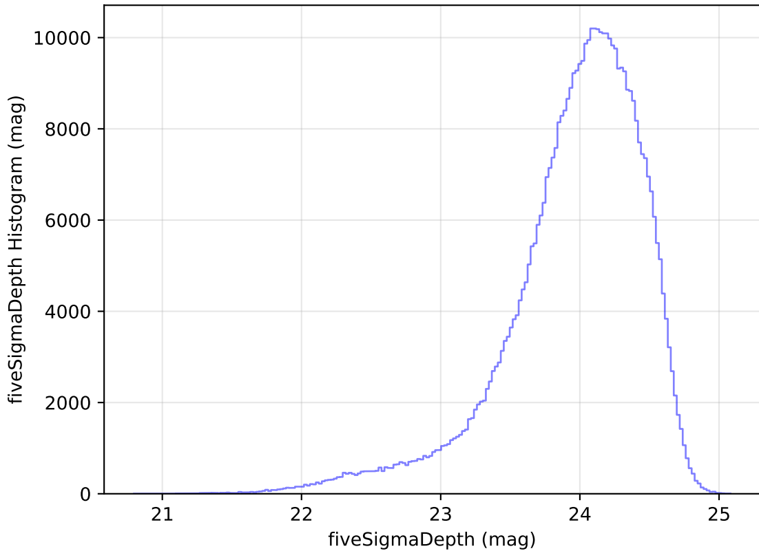
too_elab_heavy_r128_d3_griz_v3.4_10yrs WFD r band: fiveSigmaDepth Histogram
