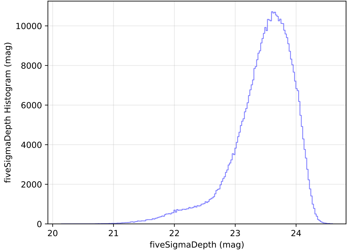
too_elab_heavy_r128_d3_griz_v3.4_10yrs WFD i band: fiveSigmaDepth Histogram
