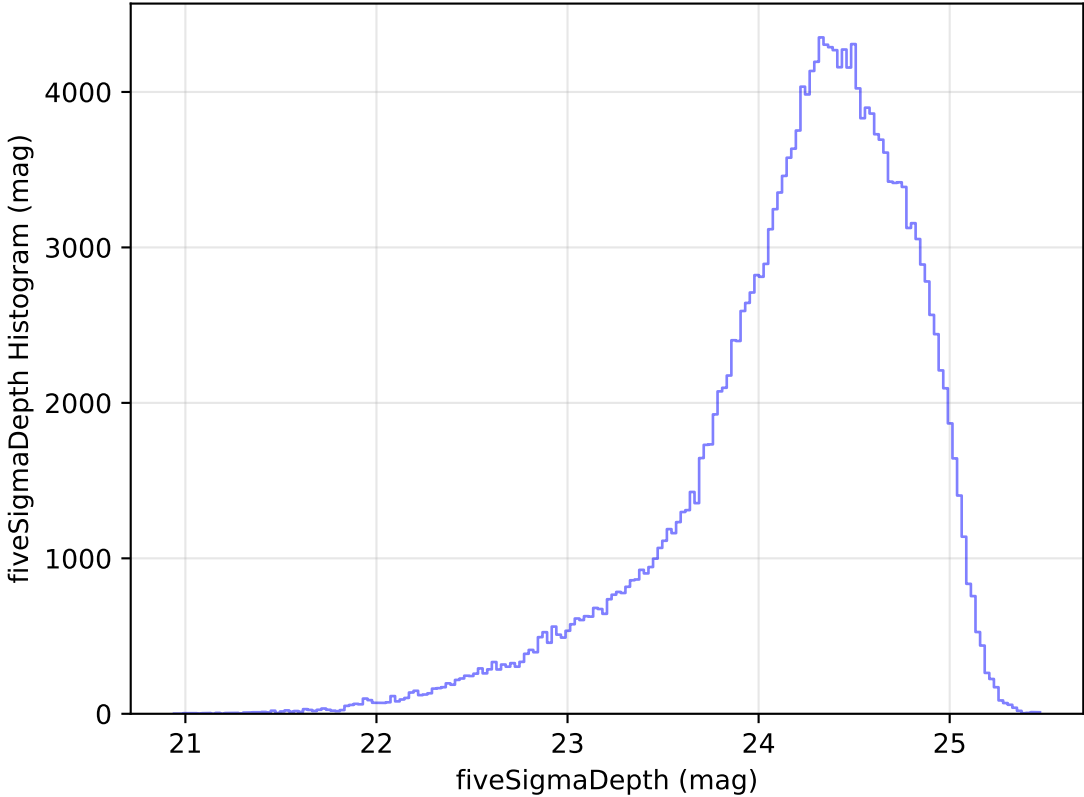
too_elab_heavy_r128_d3_griz_v3.4_10yrs WFD g band: fiveSigmaDepth Histogram
