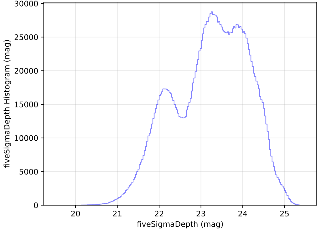
too_elab_heavy_r128_d3_griz_v3.4_10yrs WFD all bands: fiveSigmaDepth Histogram
