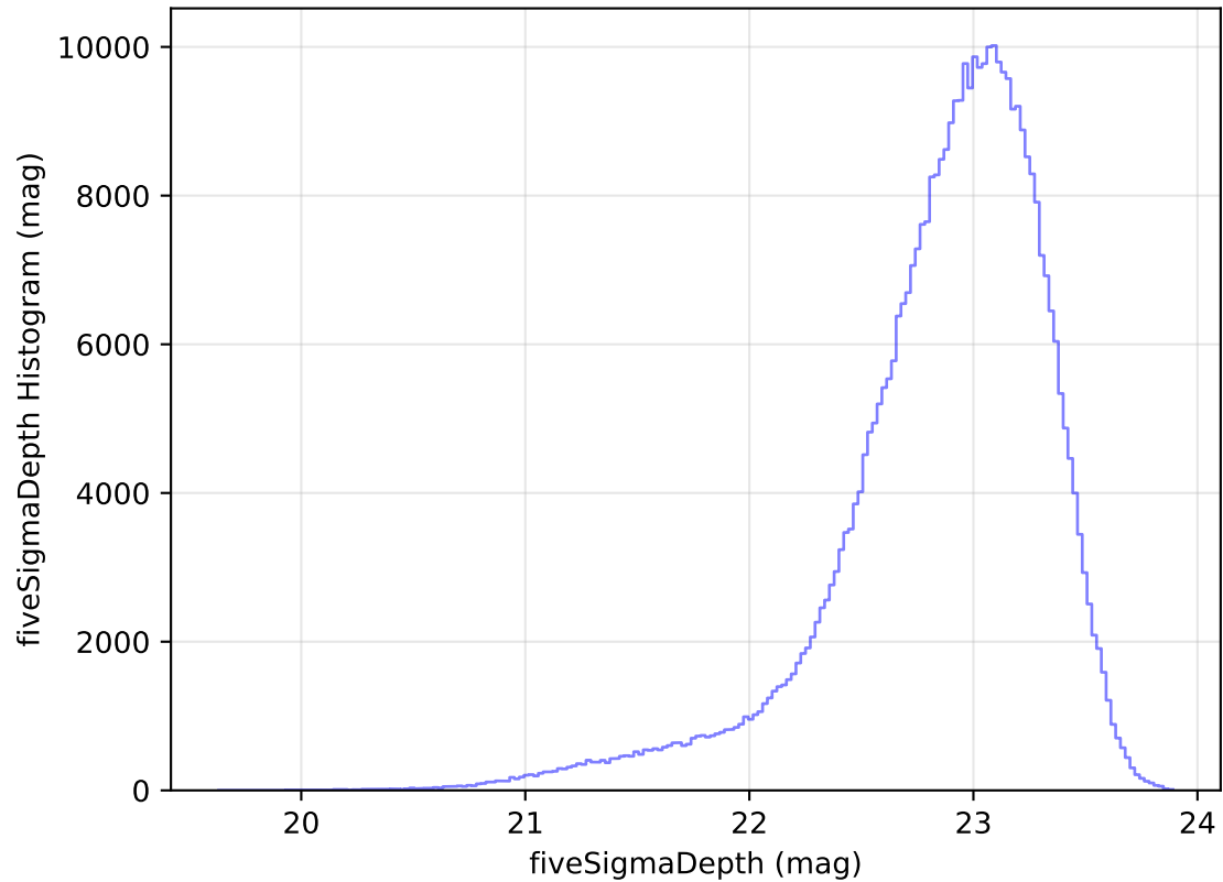
too_elab_heavy_r128_d3_griz_v3.4_10yrs All sky z band: fiveSigmaDepth Histogram
