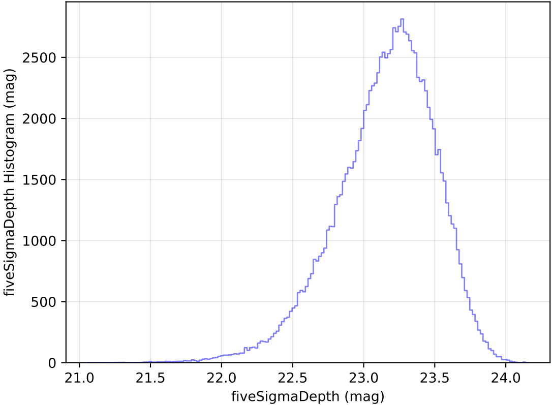
too_elab_heavy_r128_d3_griz_v3.4_10yrs All sky u band: fiveSigmaDepth Histogram
