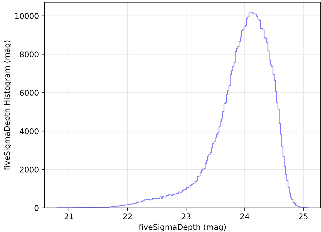
too_elab_heavy_r128_d3_griz_v3.4_10yrs All sky r band: fiveSigmaDepth Histogram
