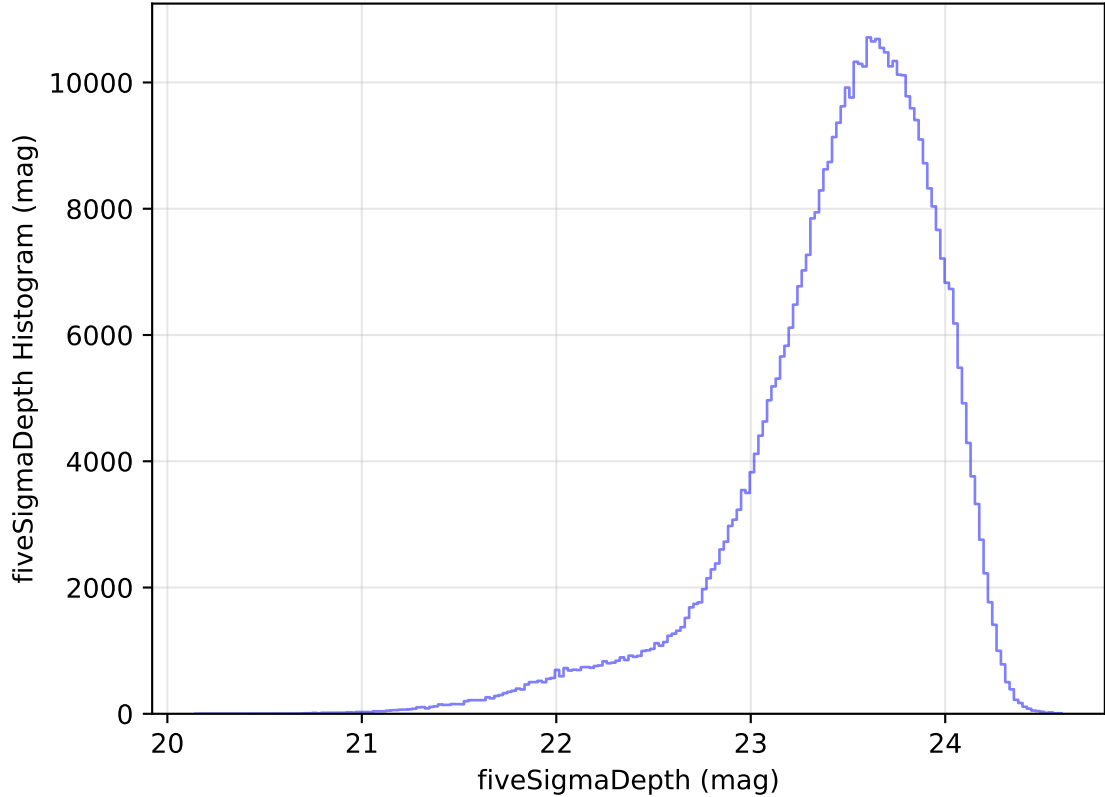
too_elab_heavy_r128_d3_griz_v3.4_10yrs All sky i band: fiveSigmaDepth Histogram
