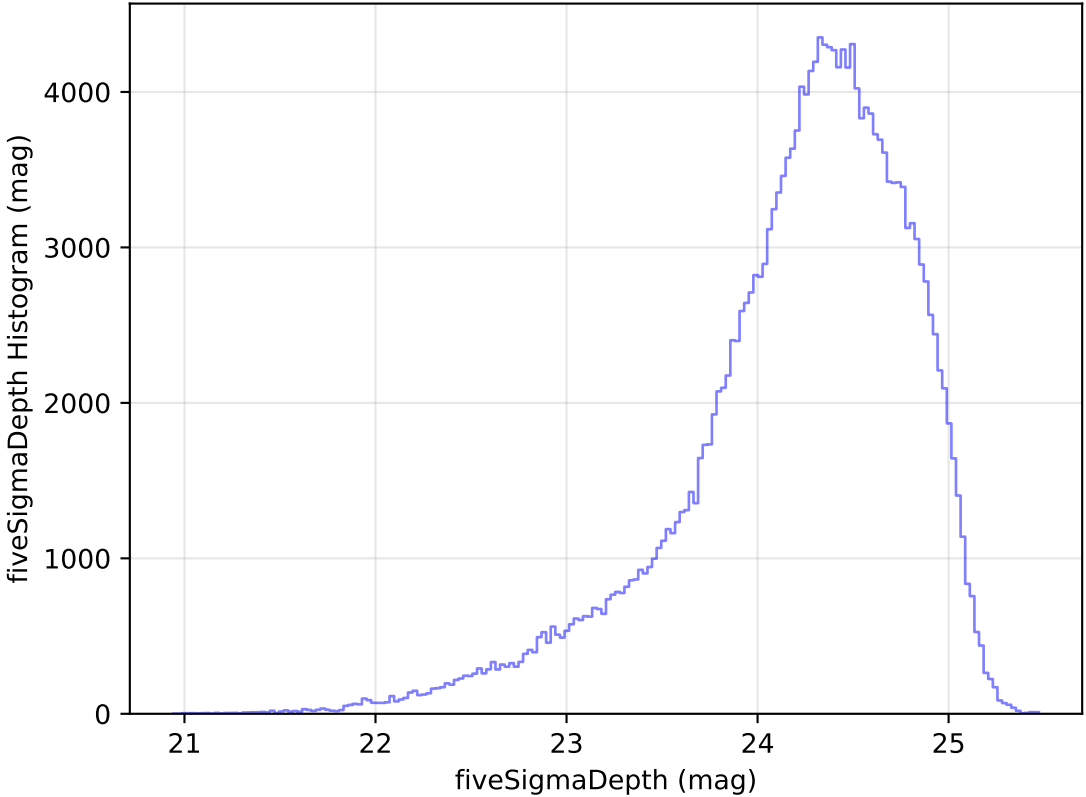
too_elab_heavy_r128_d3_griz_v3.4_10yrs All sky g band: fiveSigmaDepth Histogram
