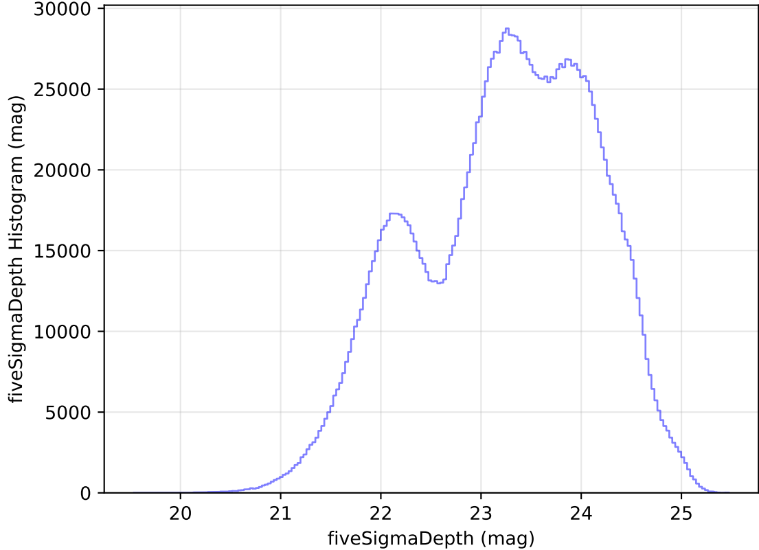
too_elab_heavy_r128_d3_griz_v3.4_10yrs All sky all bands: fiveSigmaDepth Histogram
