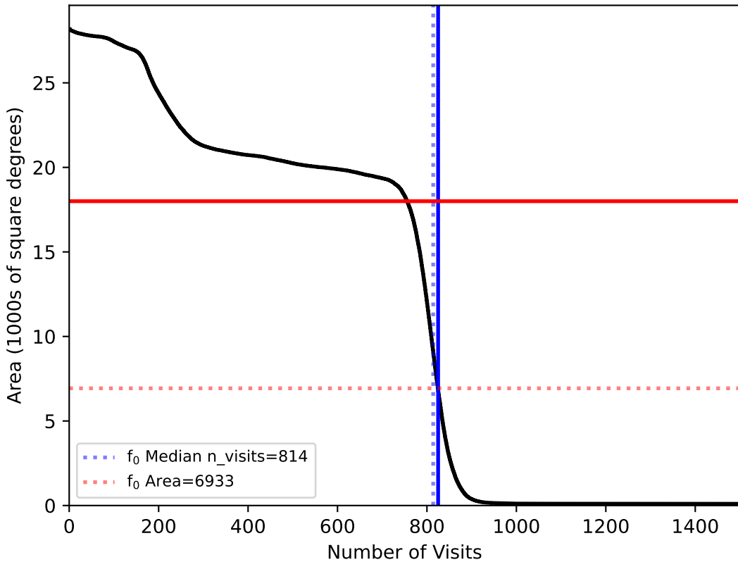
too_elab_heavy_r128_d3_griz_v3.4_10yrs All sky: fO
