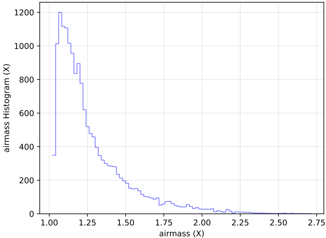
too_elab_heavy_r128_d3_griz_v3.4_10yrs Yr 1 u band: airmass Histogram
